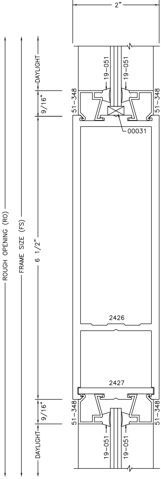
○ 6 \frac{1}{2} " INTERMEDIATE CROSSRAIL SCALE: (1=1) "
